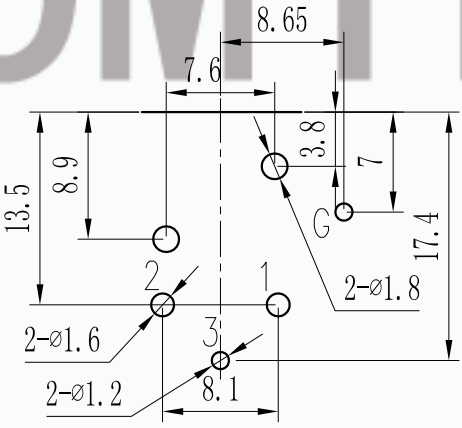
P. C. B LAYOUT (BOTTOM VIEW) Tolerance: ±0.05
