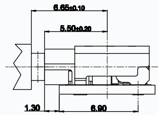
MATED CONDITION(REF.)
