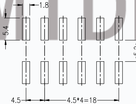
P.C.BOARD LAYOUT BOTTOM VIEW
