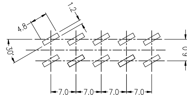
P.C.BOARD LAYOUT BOTTOM VIEW
