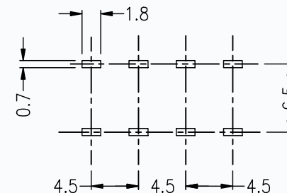
P.C.BOARD LAYOUT BOTTOM VIEW
