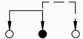
SCHEMATIC (NON-SHORTING)
