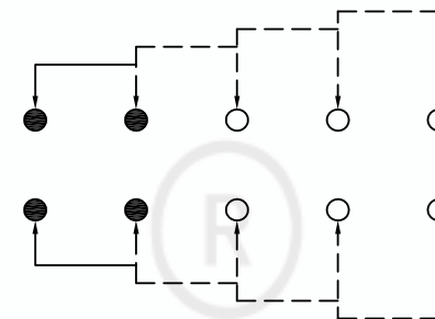
SCHEMATIC (NON-SHORTING)
