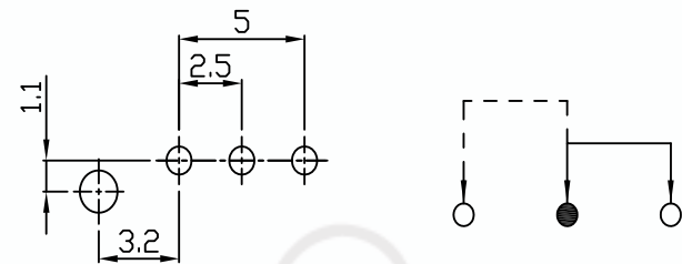
P.C.B LAYOUT CIRCUIT DIAGRAM
