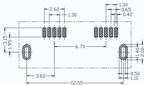
RECOMMEND PCB LAYOUT(TOP VIEW) GENERAL TOLERANCE \pm 0.05
