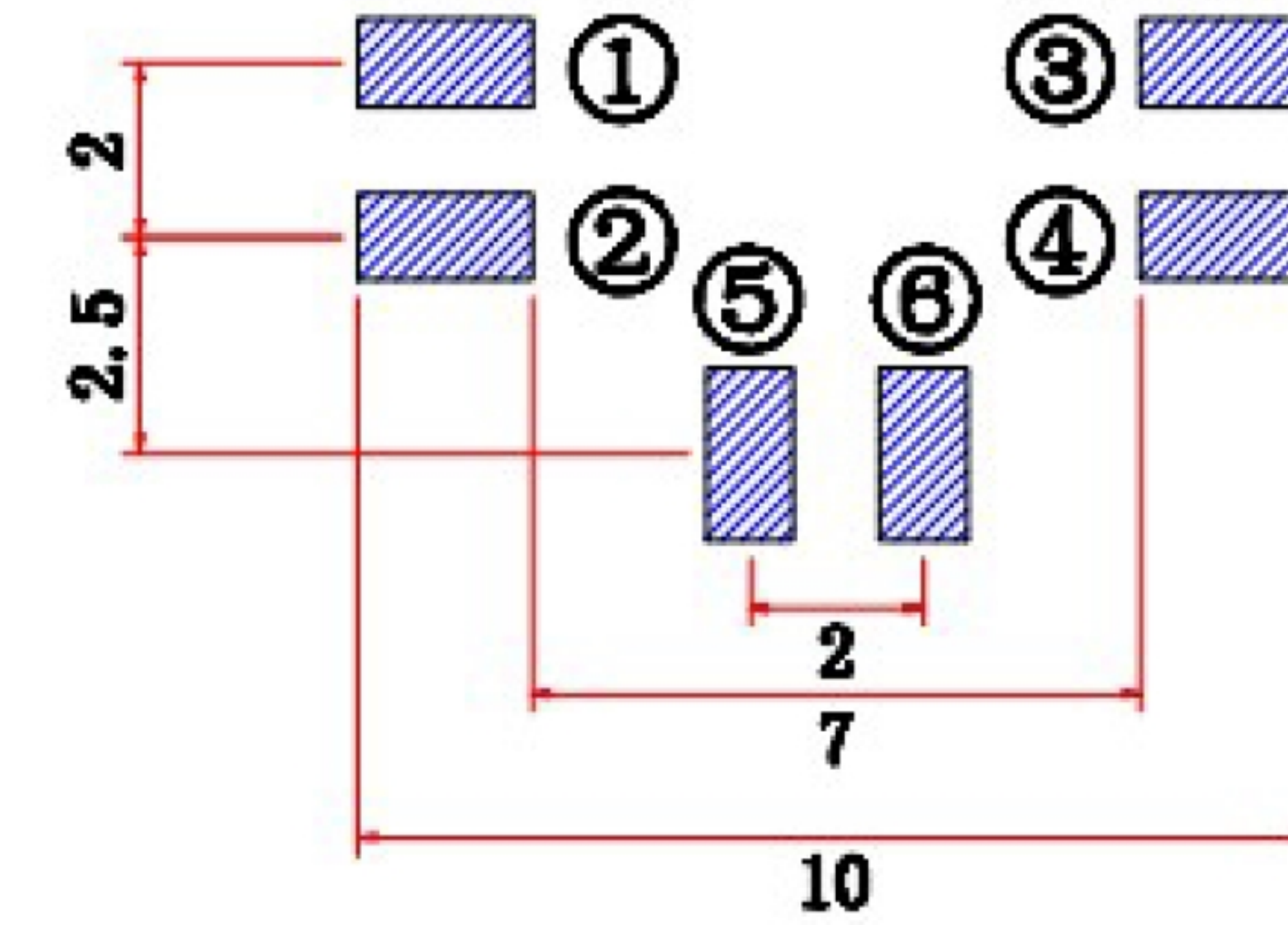
PCB LAYOT
