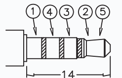
ø3.5 MATE PLUG
