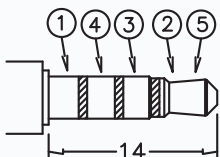
φ3.5 MATE PLUG
