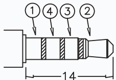
Ø3.5 MATE PLUG
