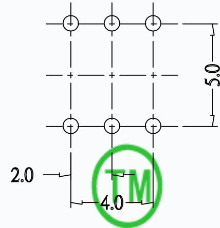
P.C.B MOUNTING PATTERN BOTTOM VIEW
