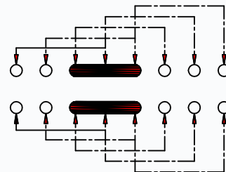
SCHMATIC (SHORTING)
