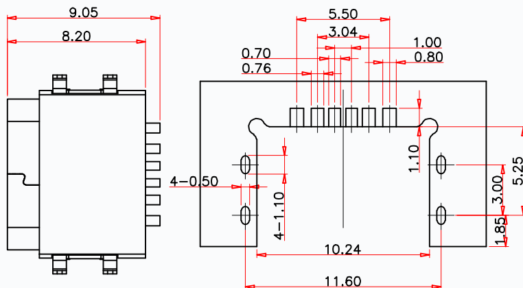
RECOMMENDED P.C.B. LAYOUT TOLERANCE UNSPECIFIED ±0.05mm
