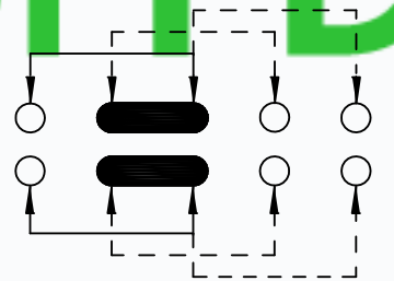
SCHEMATIC (NON-SHORTING)
