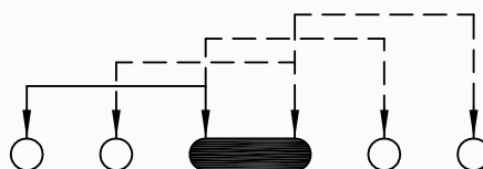
SCHEMATIC (NON-SHORTING)
