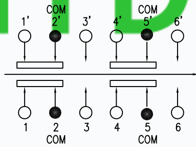
CIRCUIT DIAGRAM
